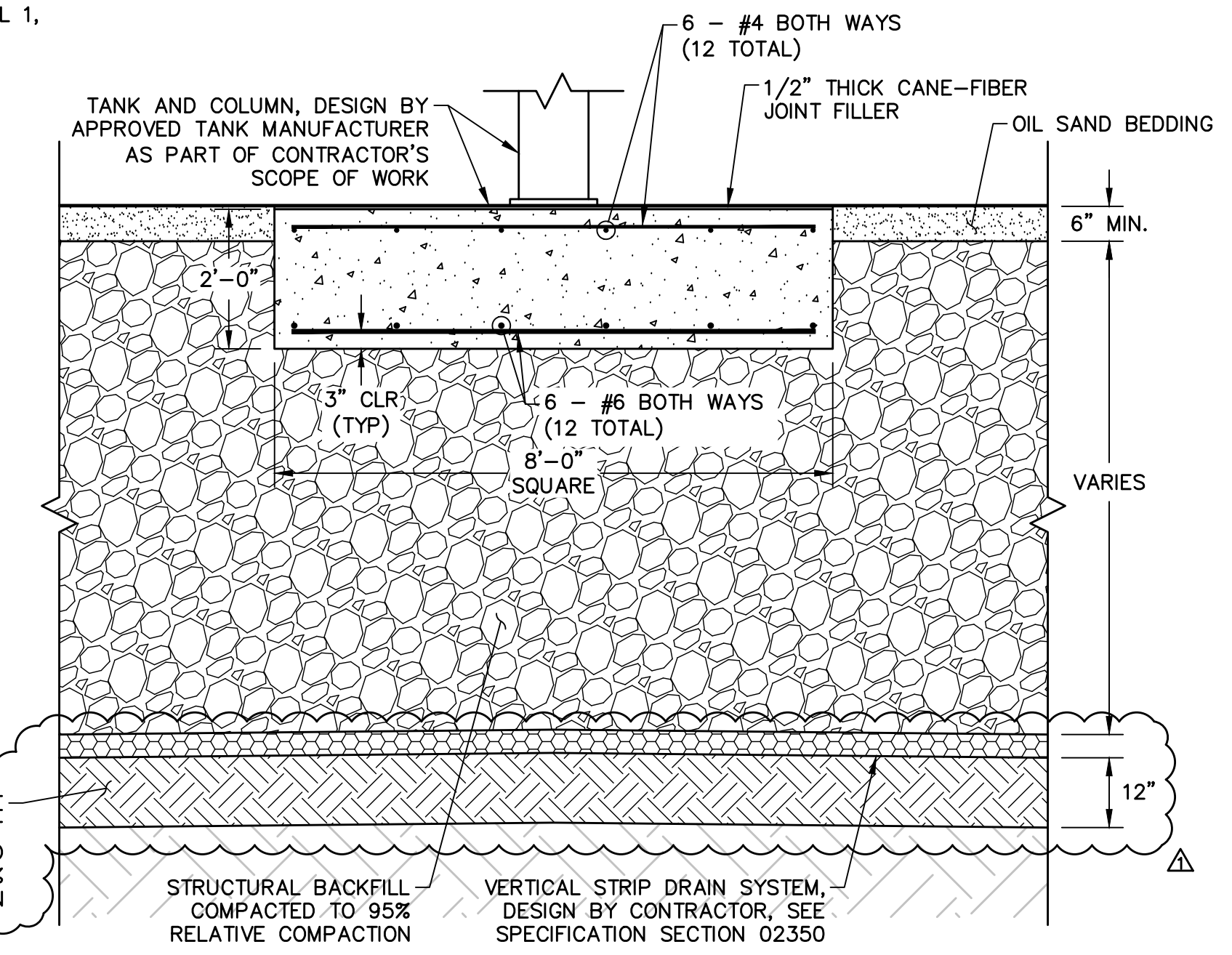
2 INTERIOR COLUMN FOUNDATION DETAIL C-03, C-05, C-06
